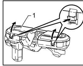
1. Wheel cover
